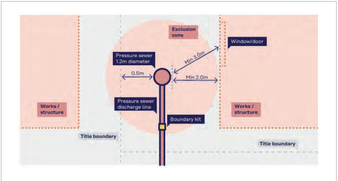
Figure 12: Clearance required to pressure sewer system components
