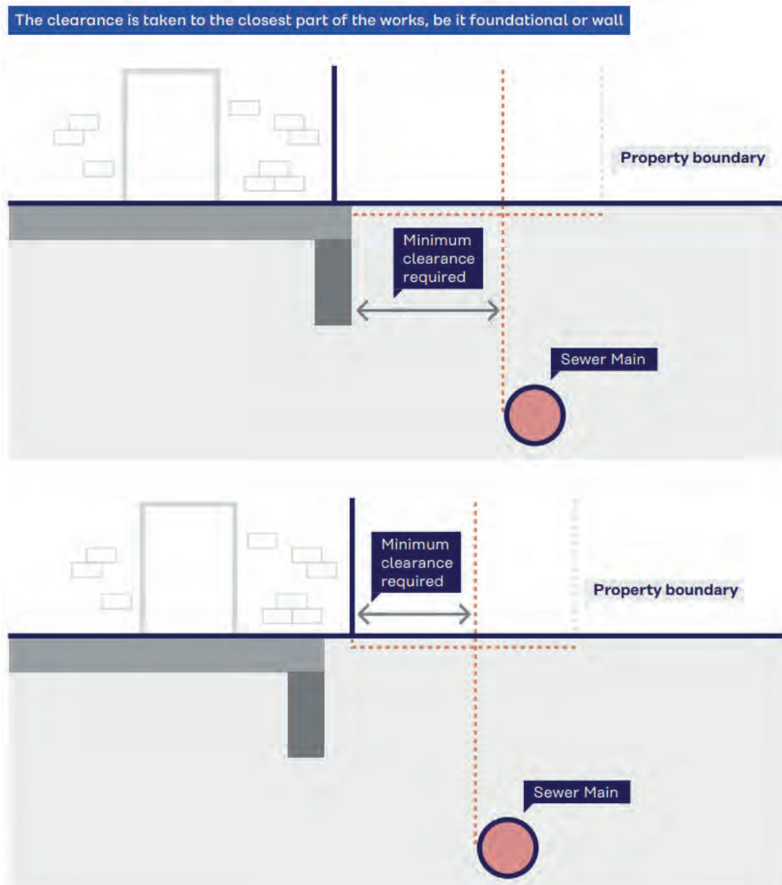
Figure 3: Clearances required from assets
