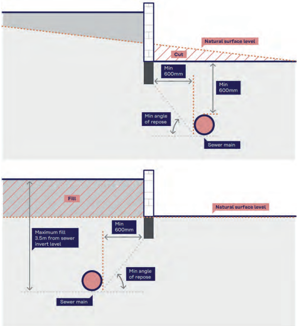
Figure 28: Excavation – cut and fill
