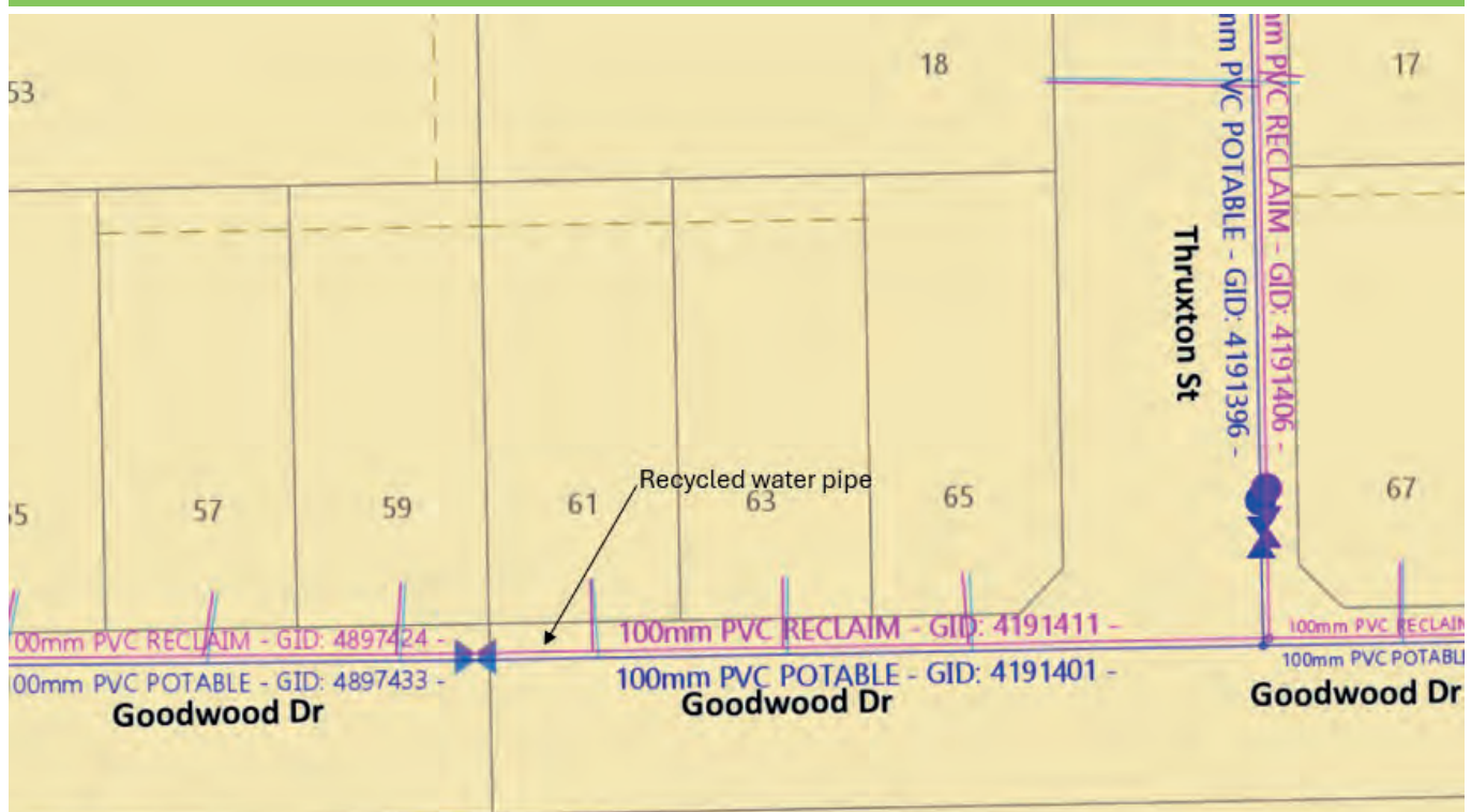
Figure 15: Recycled water asset plan
